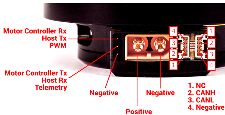
Figure 1: Connector Pin Labels
